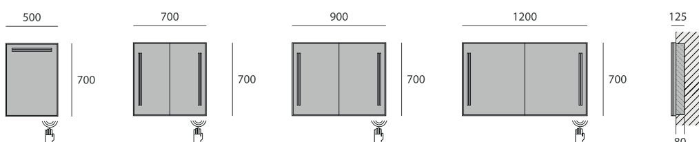
Space II Double Door Semi-recessed Cabinet 120 CL2.7012012.756.SR £1750 W1200 H700 D125mm Cut out recess: W1185 H685 D80mm
