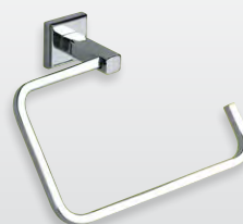
Towel Ring 6970-13 Chrome £40 W200 H145 D65mm
