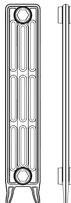
800mm High, sections 56mm
