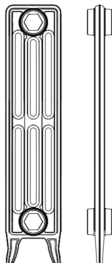
650mm High, sections 61mm
