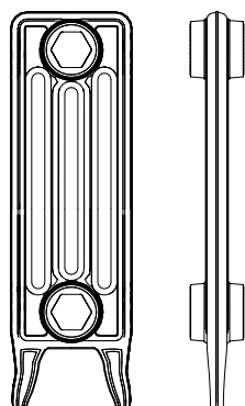
455mm High, sections 60.5mm
