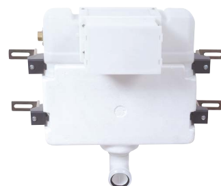
CC015 Luxury Insulated Concealed Cistern Inc Dual Flush Square Pneumatic Push Plate H36 x W50 x D15 (Tank Dimensions) • Side Inlet
