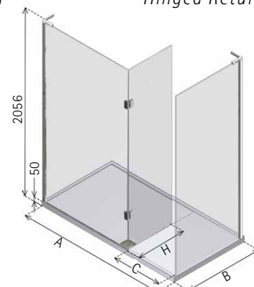
RH Entrance Hinged Return
