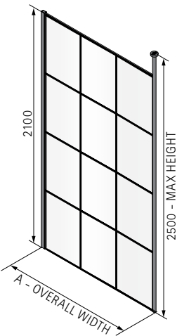
Not Handed MOWV FE Ceiling Brace Bar
